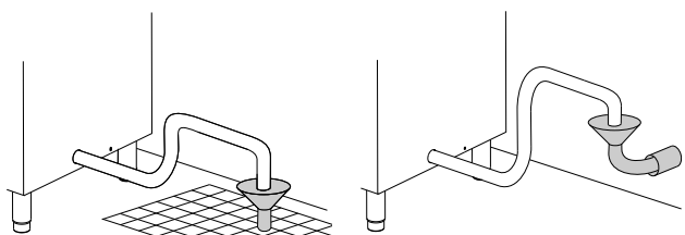
Floor discharge
